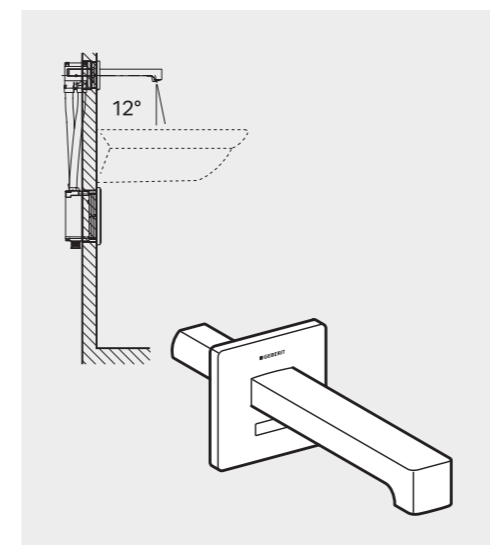
↑ Geberit washbasin tap Brenta, Wall mounting
