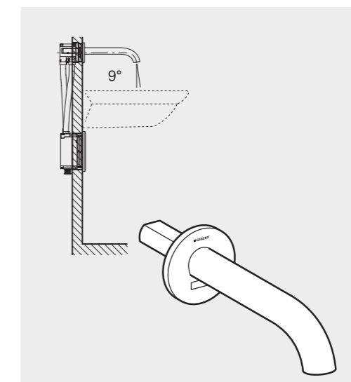
↑ Geberit washbasin tap Piave, Wall mounting
